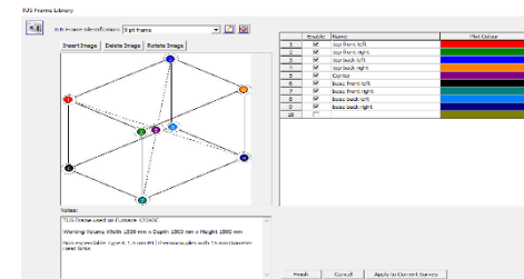
TUS frame Library files allowing clear documentation of TUS thermocouple location on TUS frame within furnace working volume.
