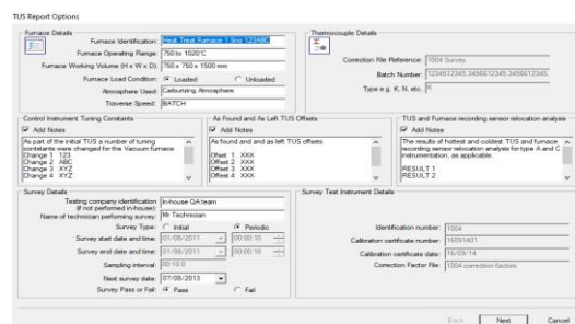
TUS report dialogue allowing customisable set-up of all information (auto and manual input) required for AMS2750G and CQI-9 report generation.
